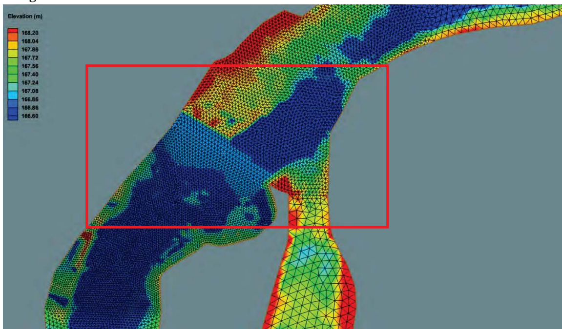
Figure 6. Assumed computation mesh for complete removal of Capes Dam used in the hydrodynamic modeling.
