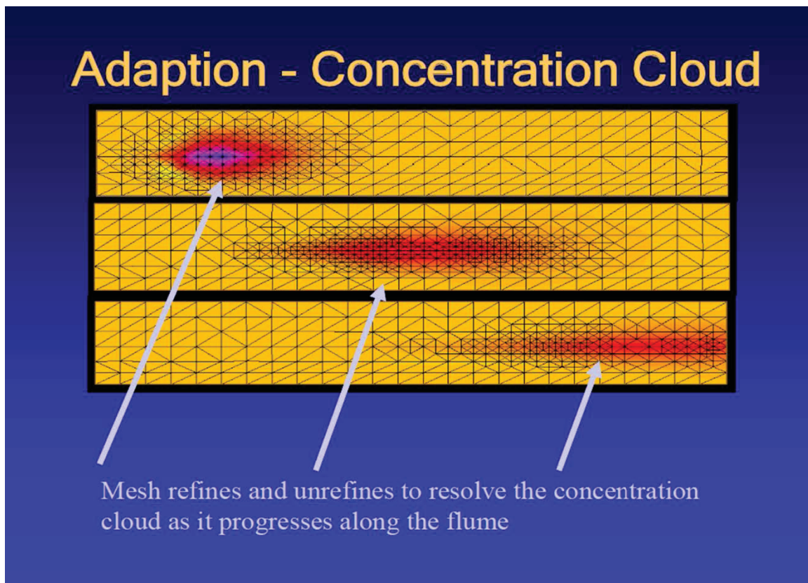
Figure 9. Example of dynamically adaptive mesh of ADH for refinement of sediment transport.
