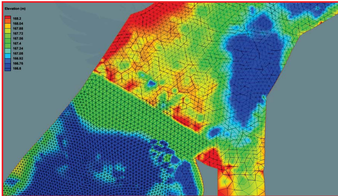
Figure 5. Assumed computation mesh for half height Capes Dam used in the hydrodynamic modeling.
