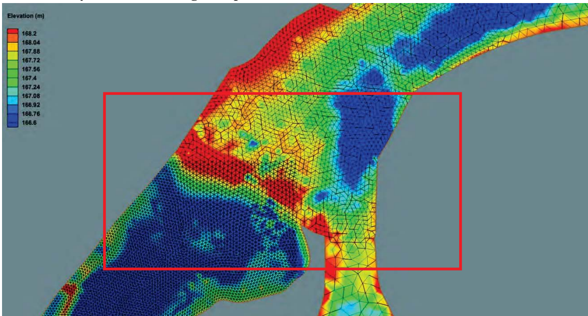
Figure 4. Assumed computation mesh for full height Capes Dam used in the hydrodynamic modeling.
