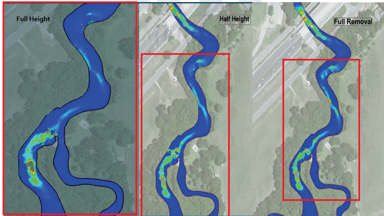
Figure 10. Computed bed shear stress at 300 cfs for each of the dam scenarios.
