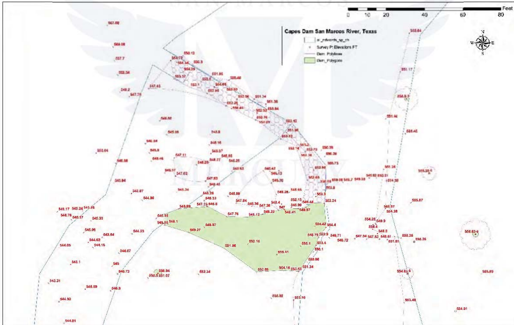
Figure 3. Survey data for full height Capes Dam.
