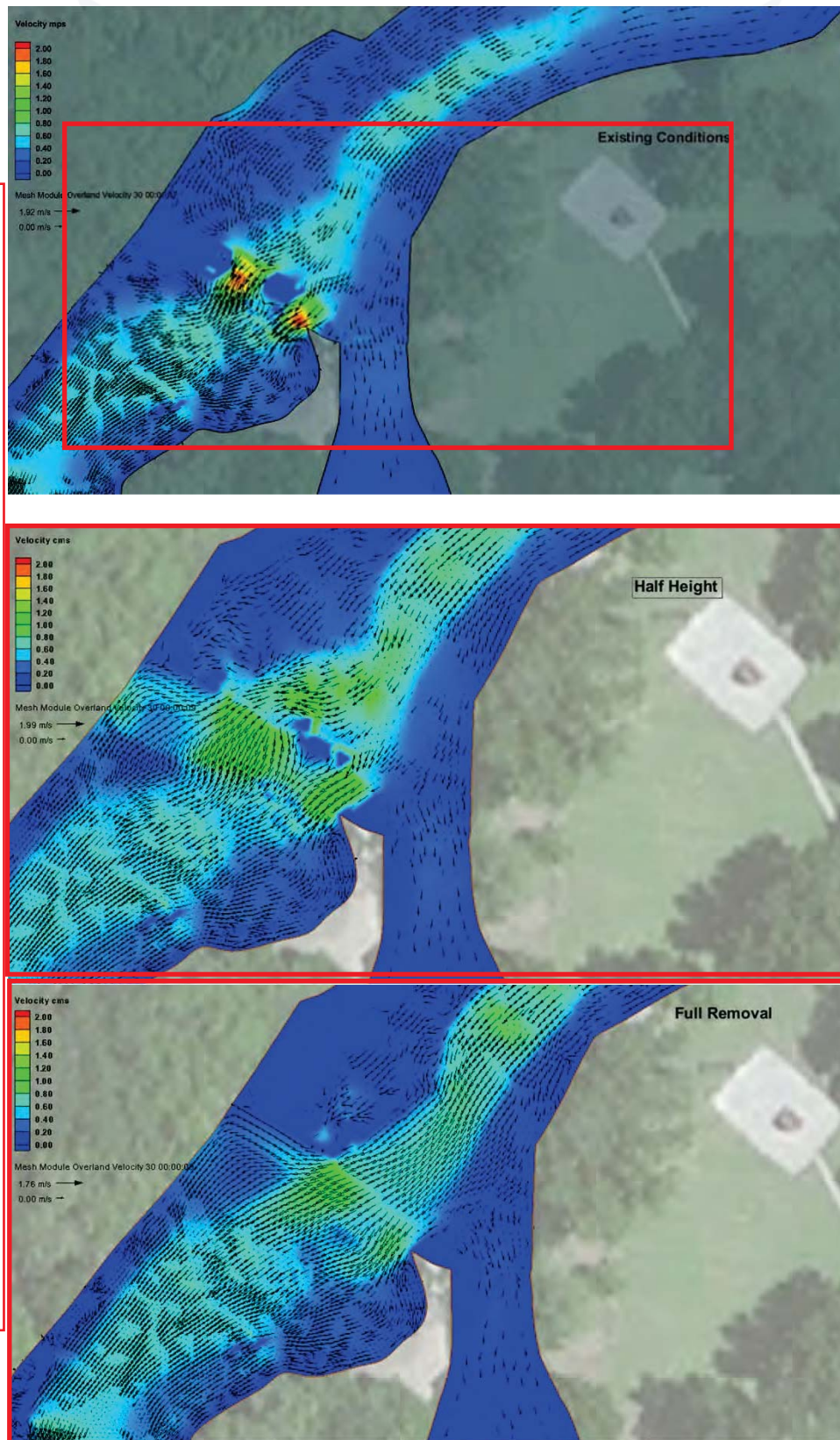
Figure 11. Velocity magnitude and directions at 300 cfs under full height, half height and full dam removal.
