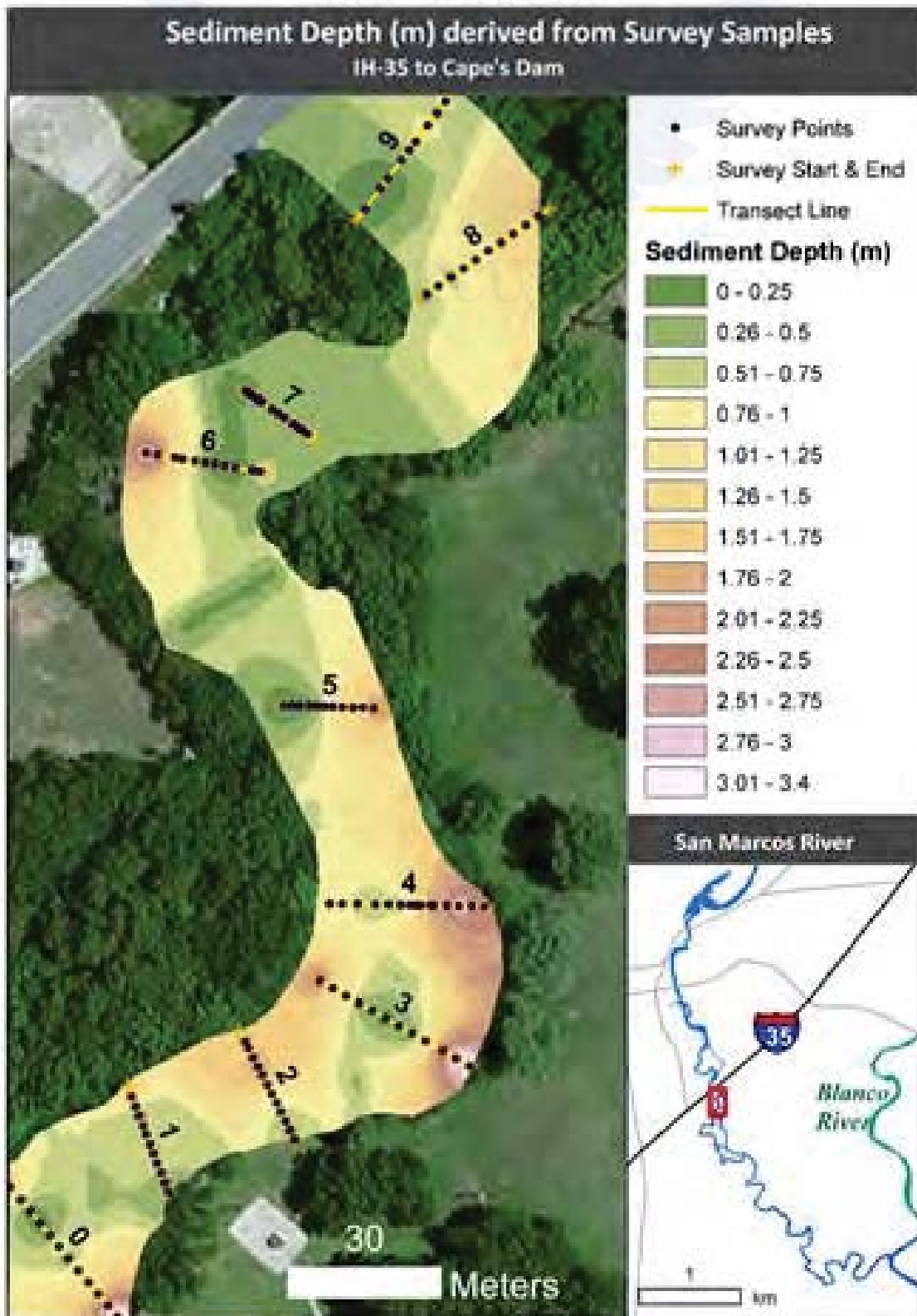
Figure 7. Location of field measurements of sediment behind Capes Dam and interpolated spatial distribution used in the hydrodynamic modeling (adapted from Hudson 2012).
