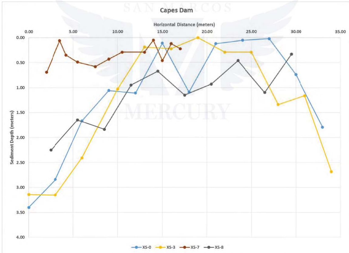
Figure 8. Sediment depth profiles for selection cross sections (see Figure 7 for location) behind Capes Dam (adapted from Hudson 2012).
