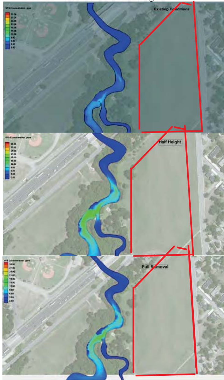
Figure 12. Mobility of fine sediments at 300 cfs under full, half height, and full removal of Capes Dam.
