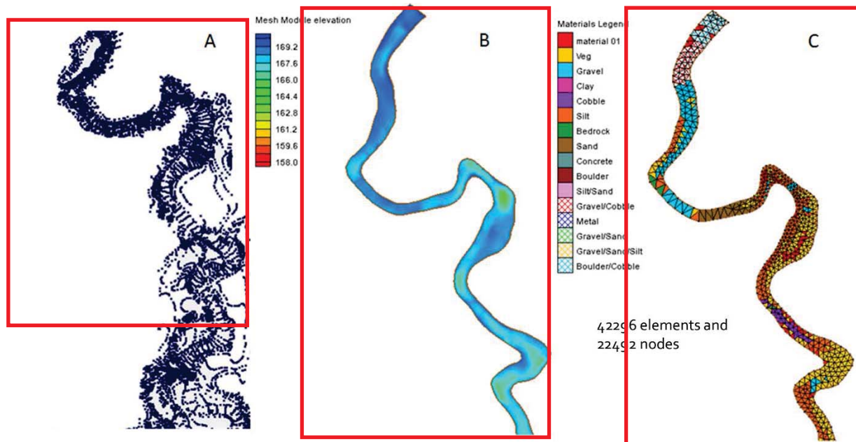
Figure 3. Example of field measured topography points (A) and computational mesh mapped onto elevation contours (B) and substrate (C).
